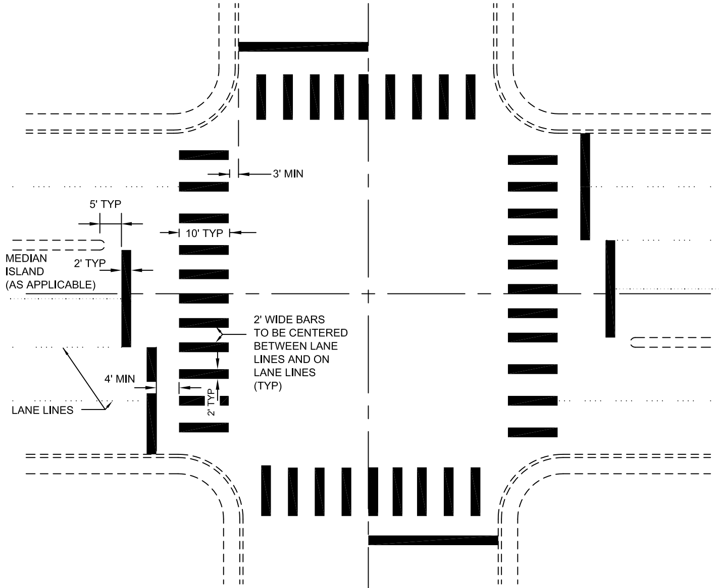
TYPICAL CROSSWALK STRIPING DETAIL
