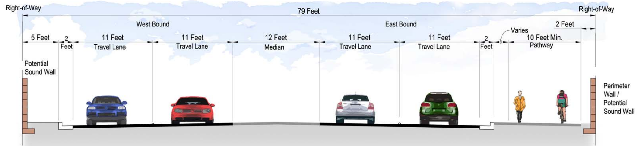
RAINBOW ALTERNATIVE TYPICAL ROADWAY SECTION ARIZONA SIDE
