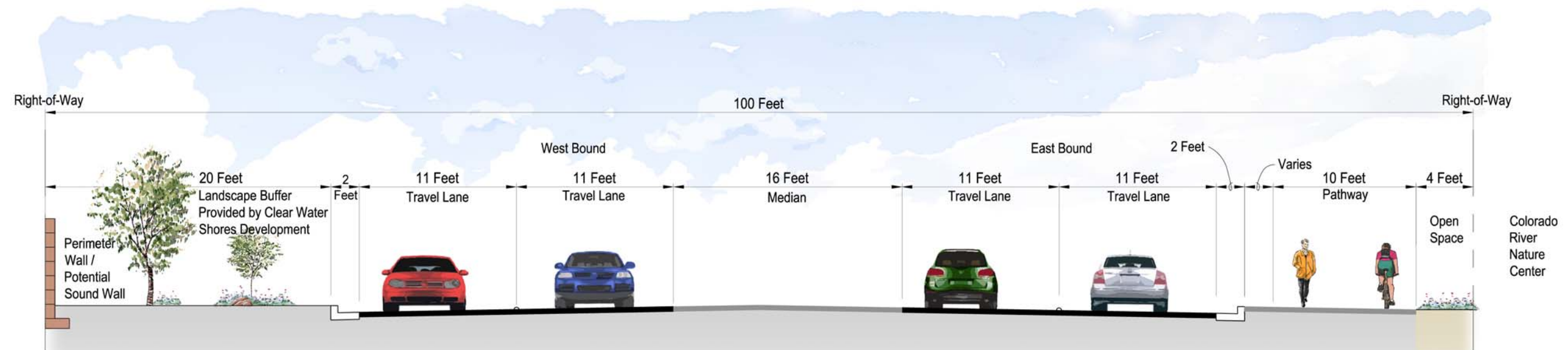
PARKWAY ALTERNATIVE TYPICAL ROADWAY SECTION ARIZONA SIDE
